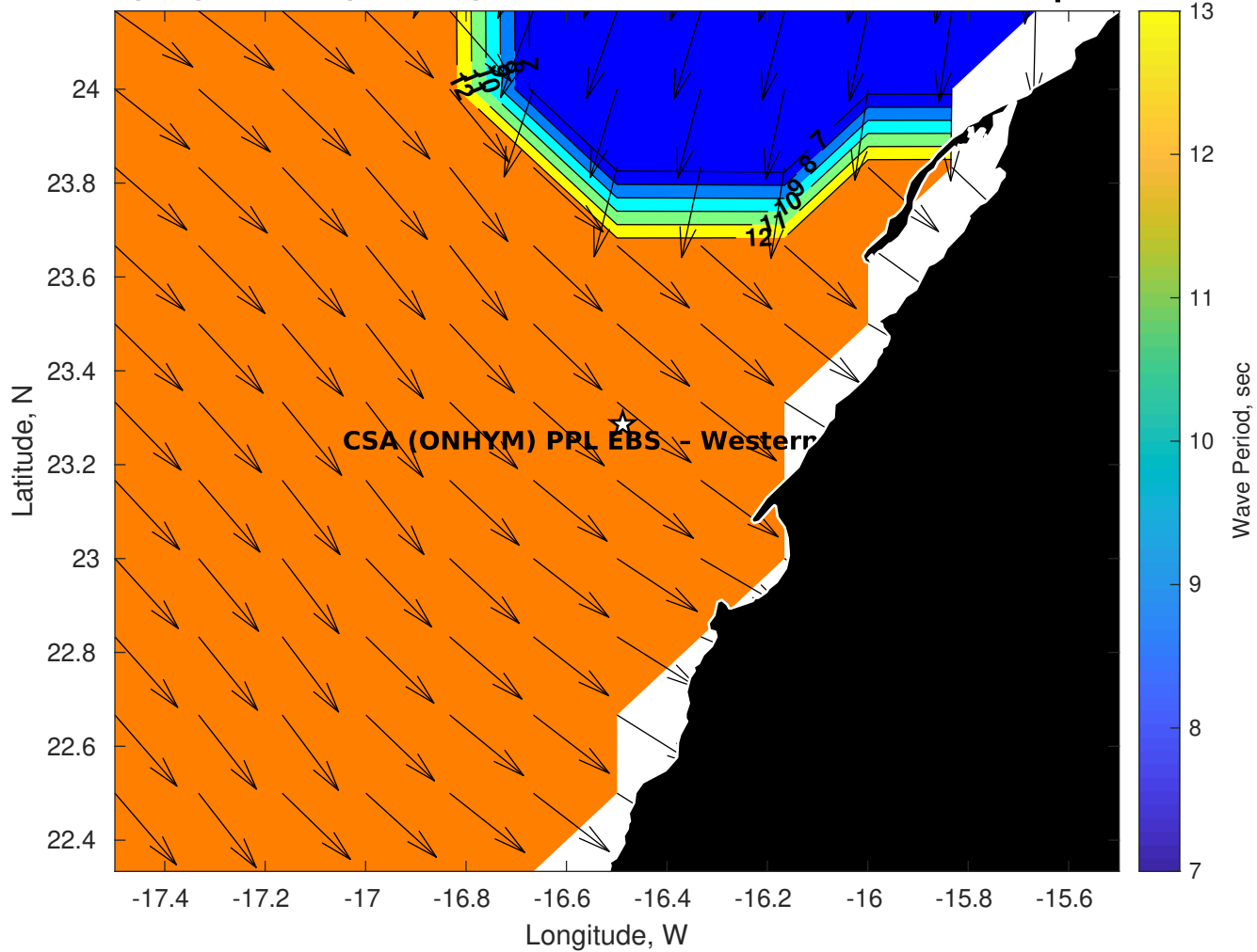
Wave Period (sec) for CSA (ONHYM) PPL EBS - Western Sahara at 17-Sep-2025 09:00:00
