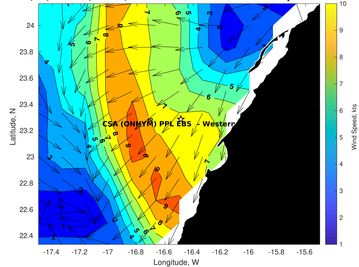
Winds (kts) for CSA (ONHYM) PPL EBS - Western Sahara at 17-Sep-2025 09:00:00
