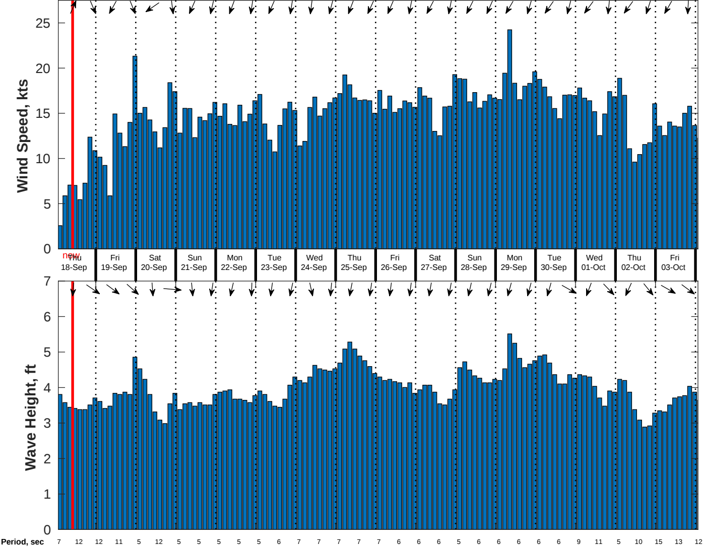
Wind & Wave Forecast for CSA (ONHYM) PPL EBS - Western Sahara from 17-Sep-2025 01:00:00 to 03-Oct-2025 01:00:00
