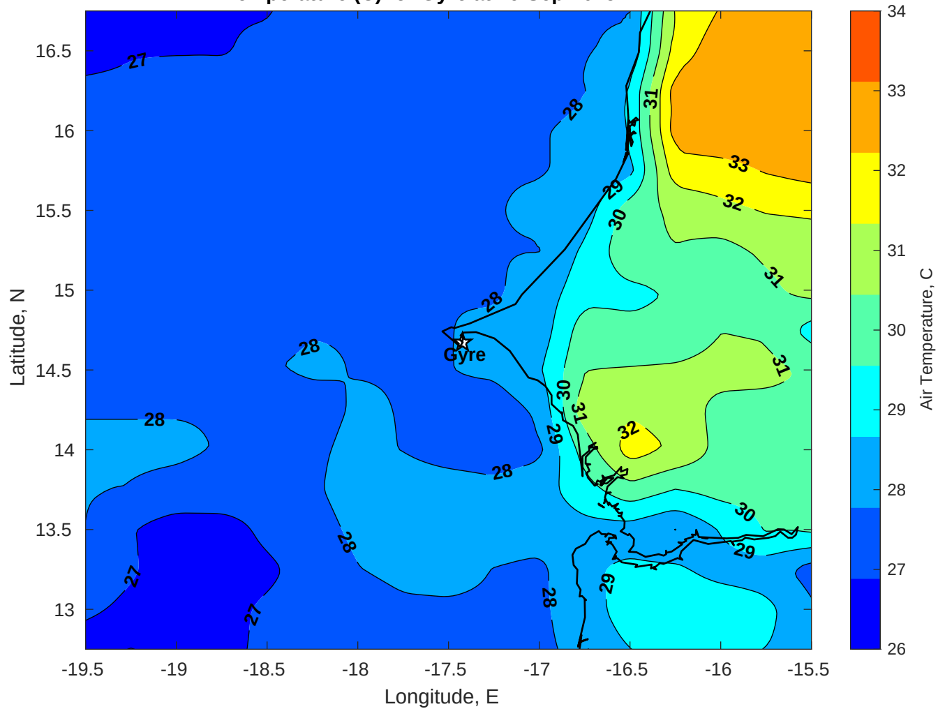
Air Temperature (C) for Gyre at 16-Sep-2025
