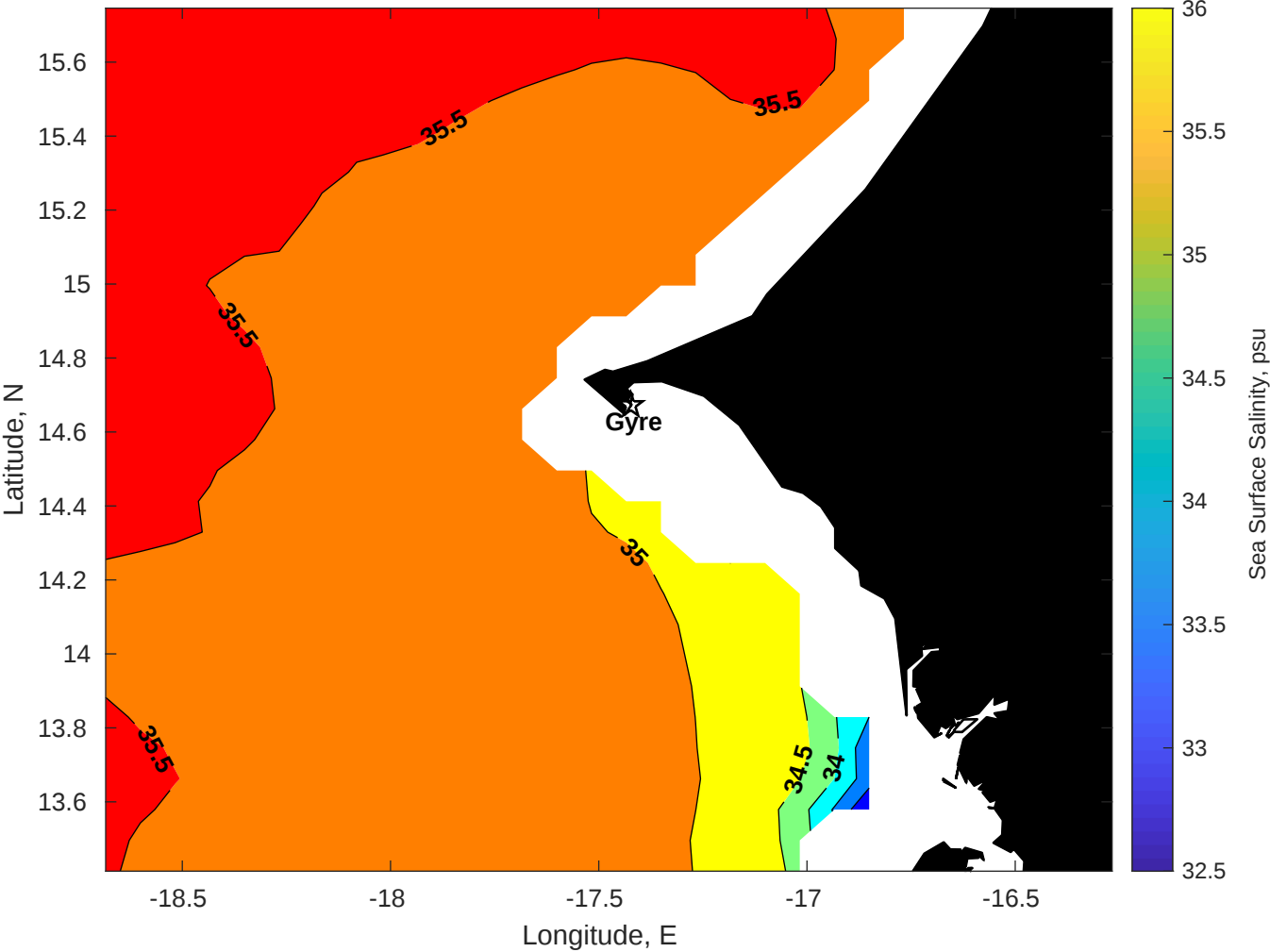
Surface Salinity for Gyre at 16-Sep-2025 00:00:00
