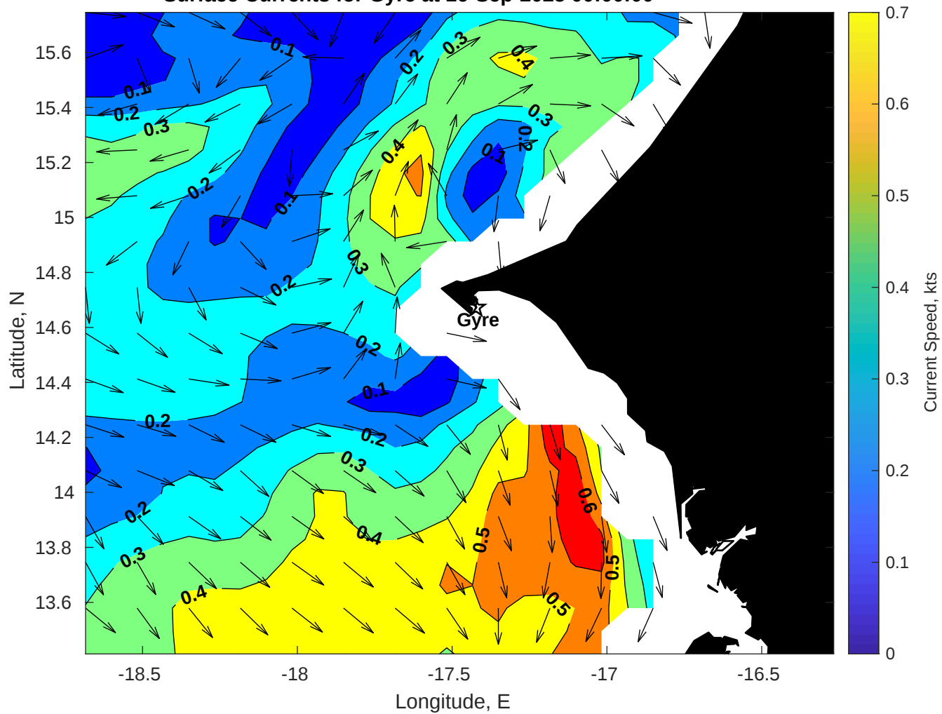
Surface Currents for Gyre at 16-Sep-2025 00:00:00
