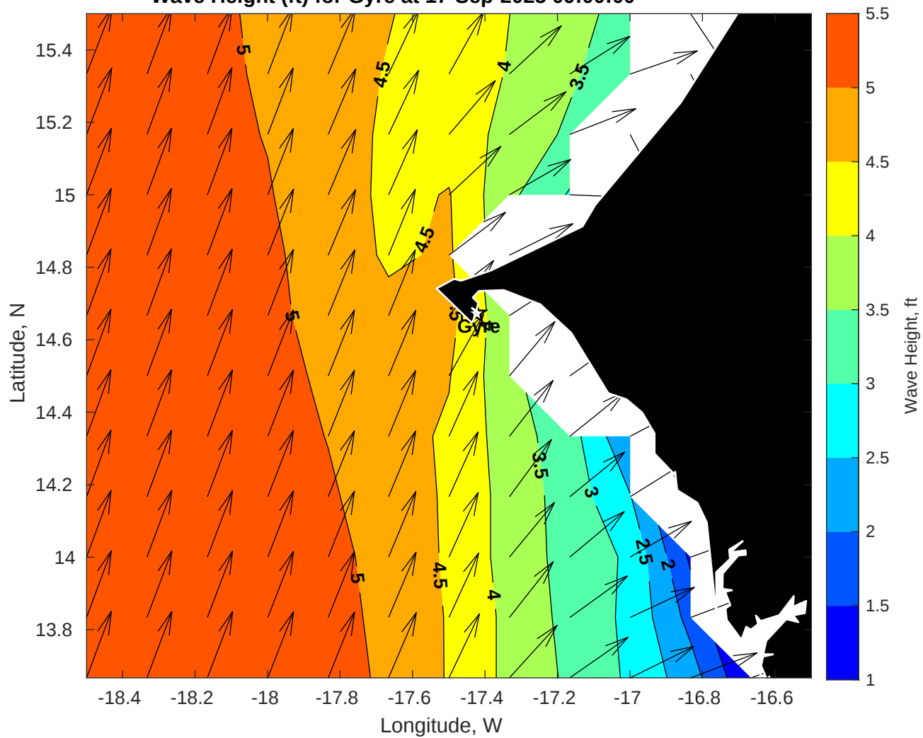
Wave Height (ft) for Gyre at 17-Sep-2025 09:00:00
