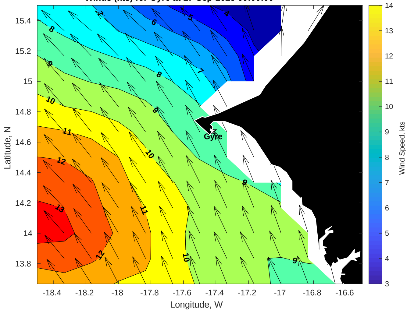
Winds (kts) for Gyre at 17-Sep-2025 09:00:00
