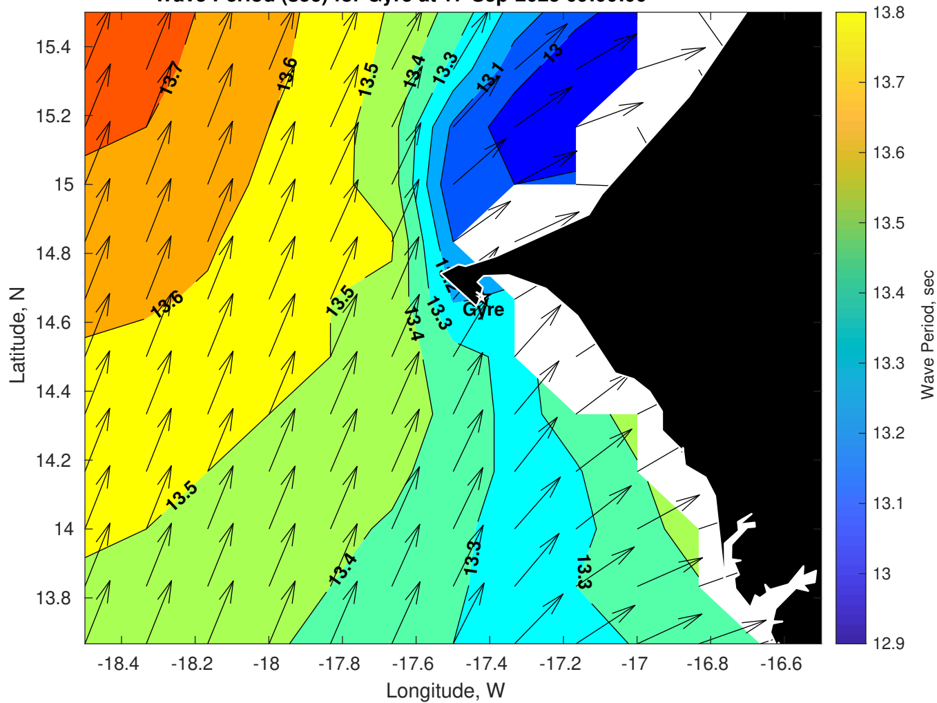
Wave Period (sec) for Gyre at 17-Sep-2025 09:00:00
