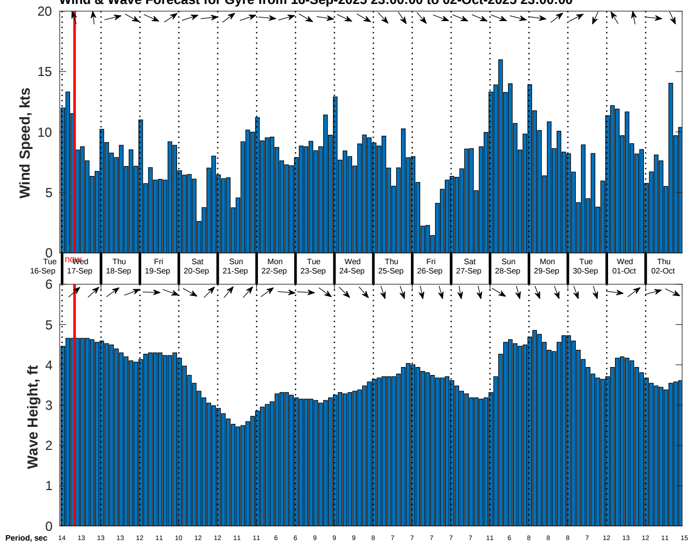
Wind & Wave Forecast for Gyre from 16-Sep-2025 23:00:00 to 02-Oct-2025 23:00:00
