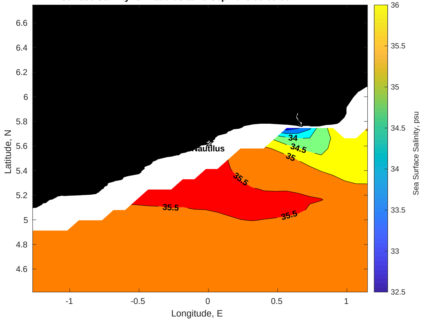
Surface Salinity for Nautilus at 16-Sep-2025 00:00:00
