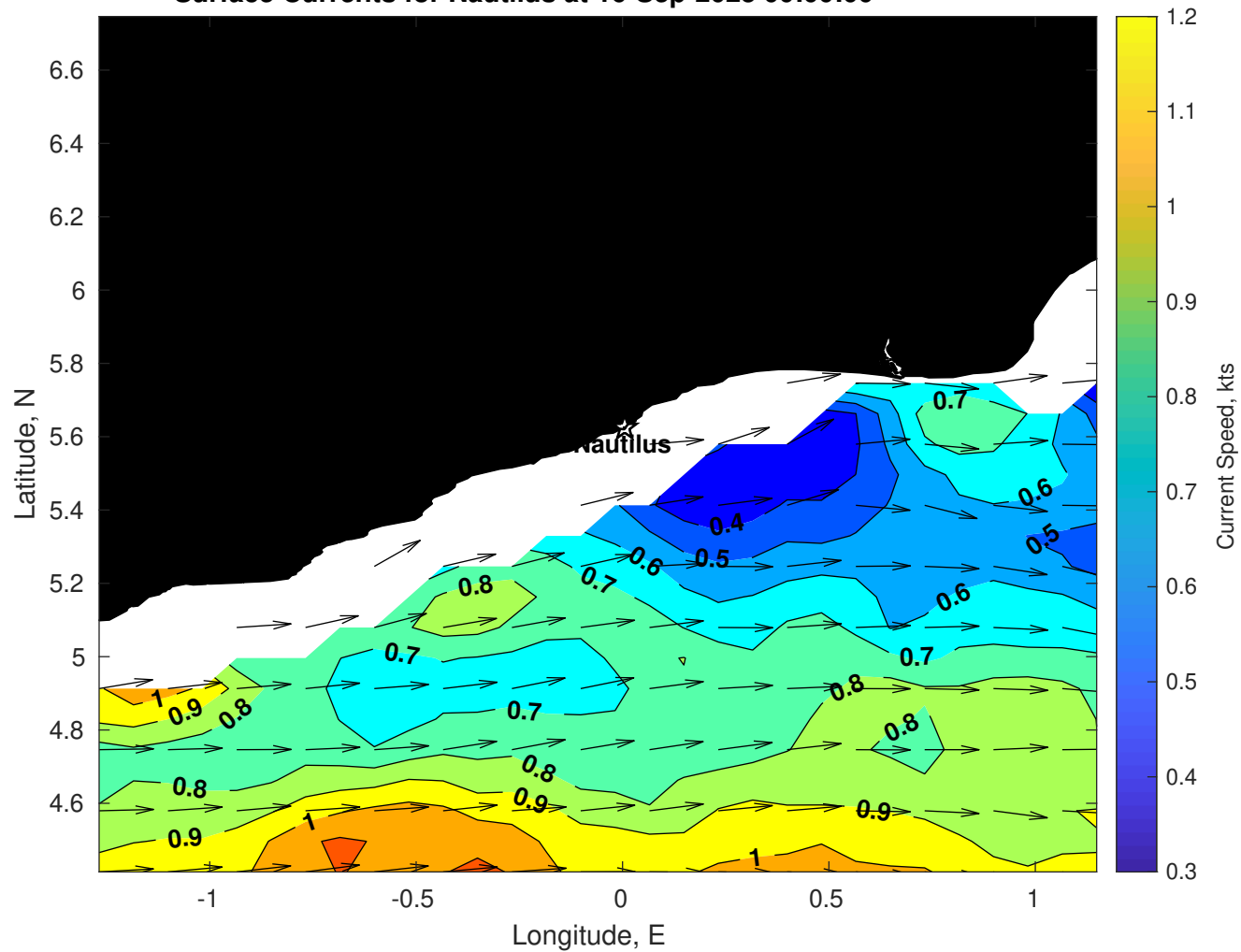
Surface Currents for Nautilus at 16-Sep-2025 00:00:00
