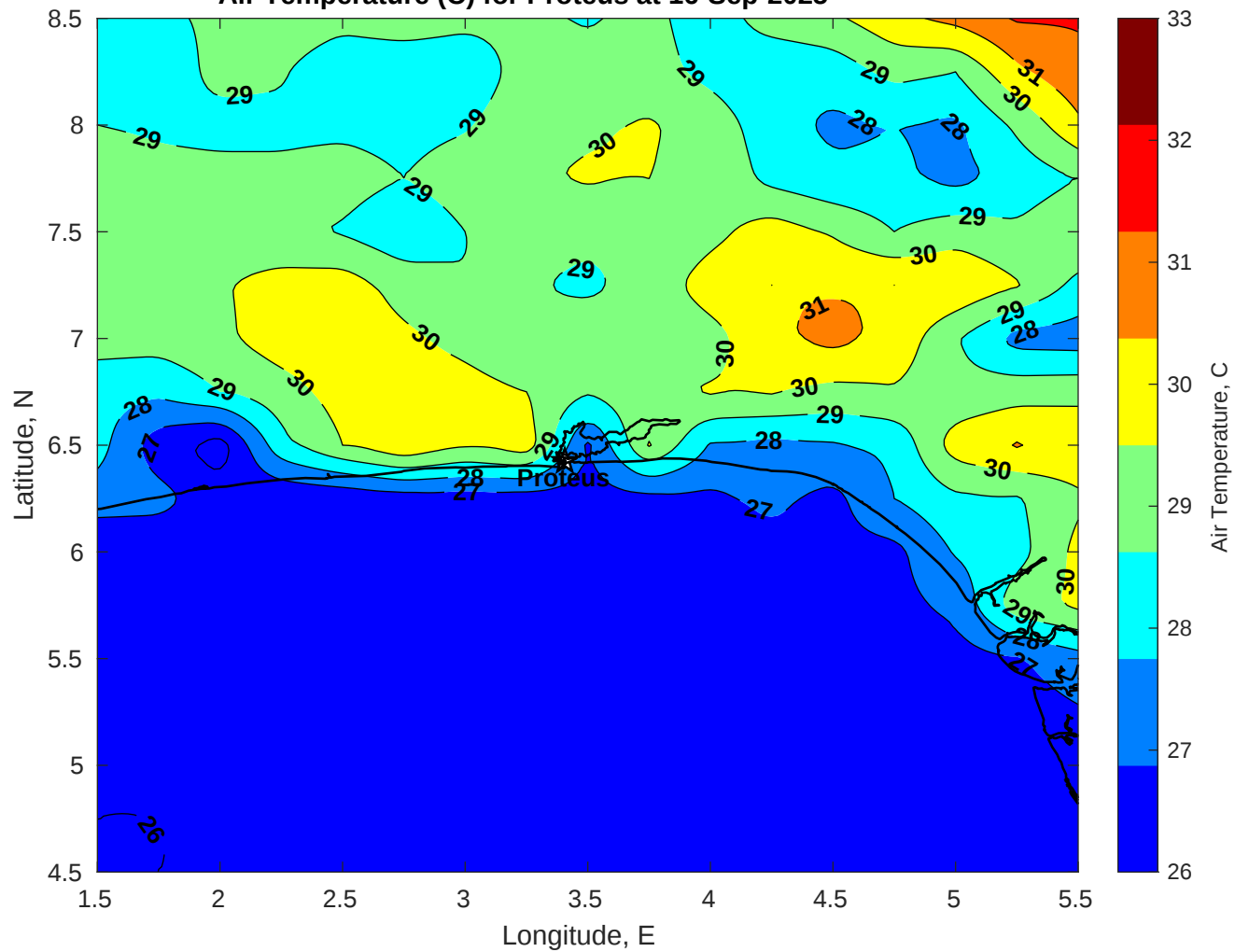
Air Temperature (C) for Proteus at 16-Sep-2025
