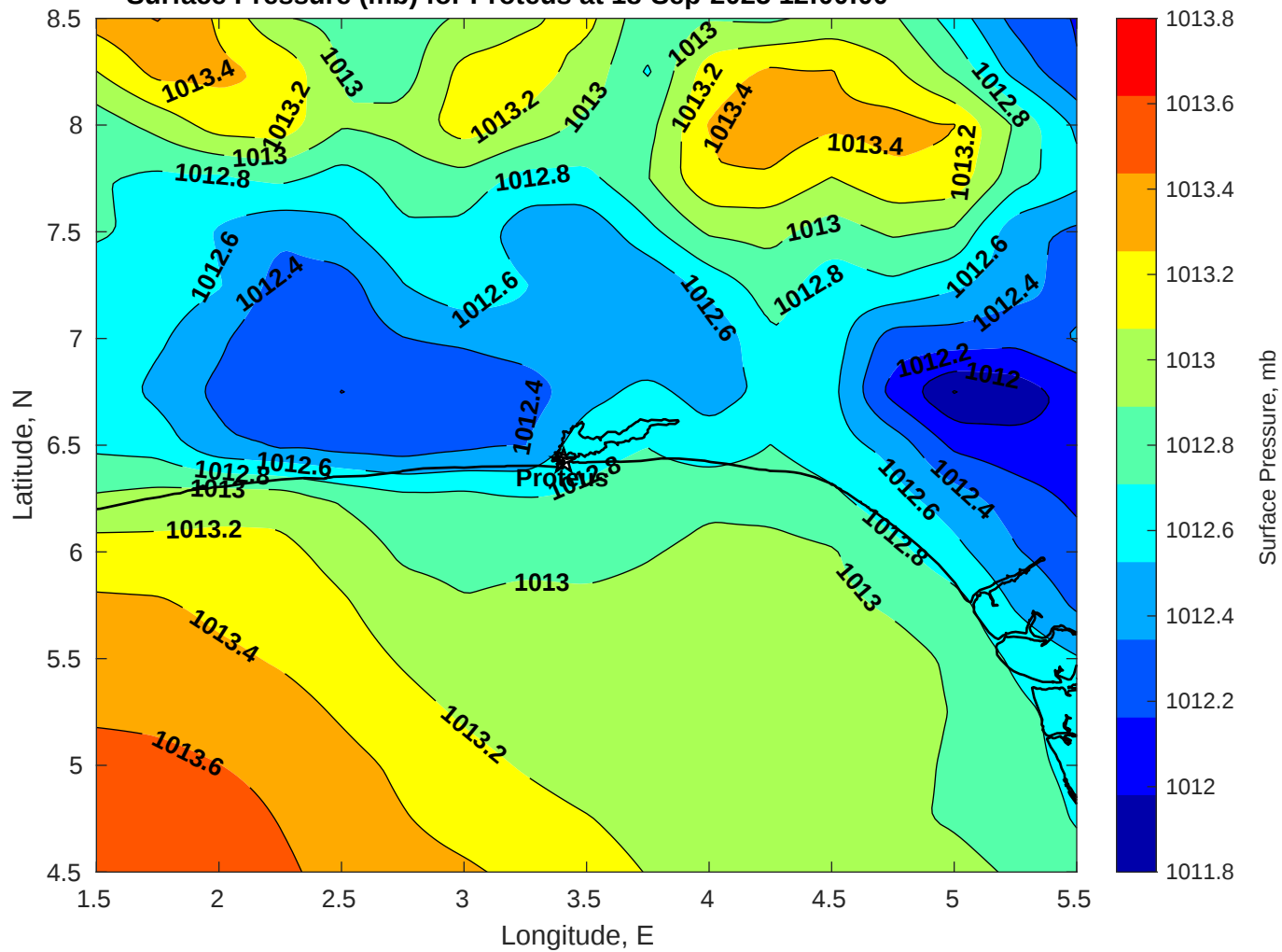
Surface Pressure (mb) for Proteus at 18-Sep-2025 12:00:00
