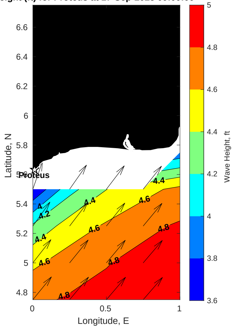
Wave Height (ft) for Proteus at 17-Sep-2025 09:00:00
