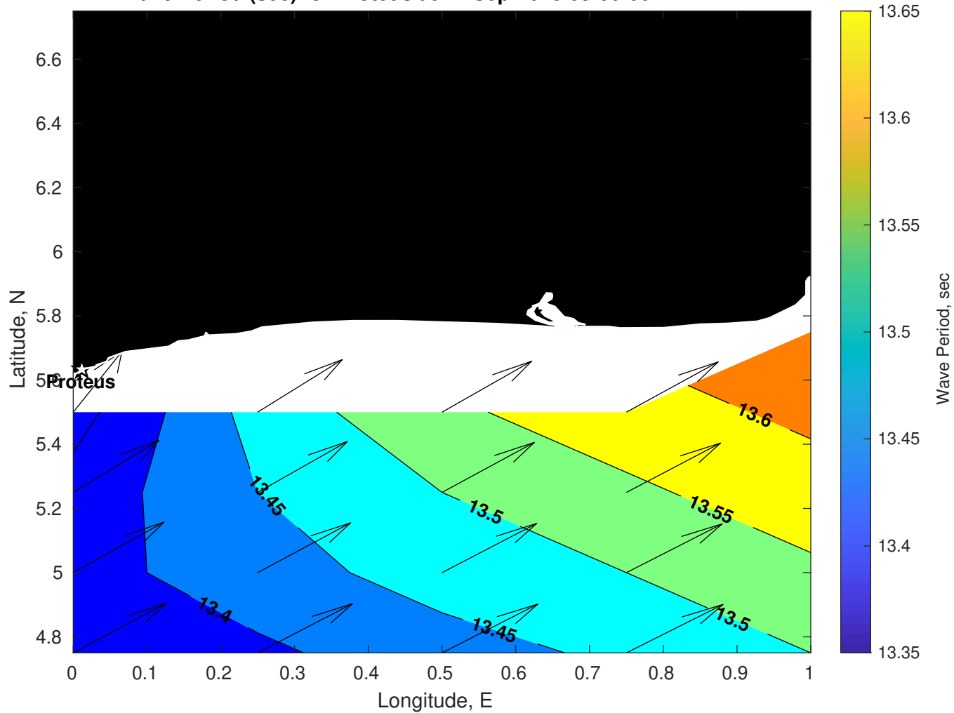
Wave Period (sec) for Proteus at 17-Sep-2025 09:00:00
