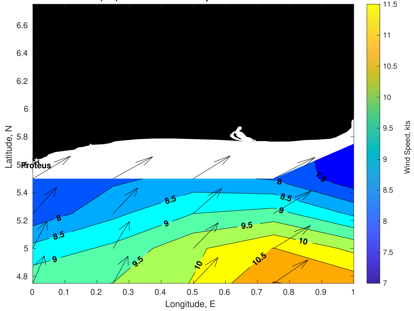
Winds (kts) for Proteus at 17-Sep-2025 09:00:00
