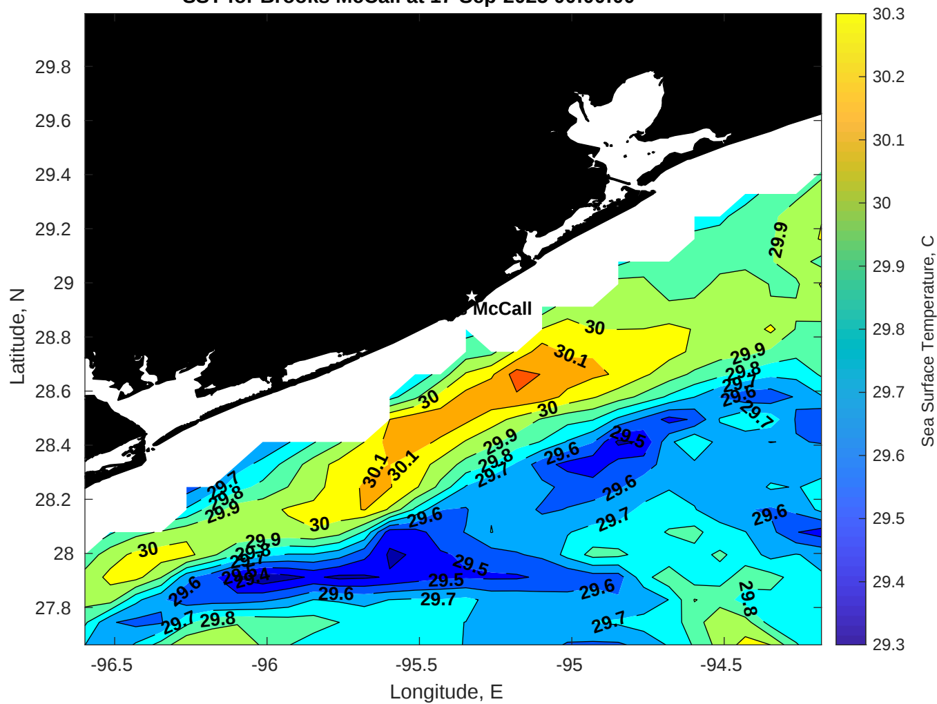
SST for Brooks McCall at 17-Sep-2025 00:00:00
