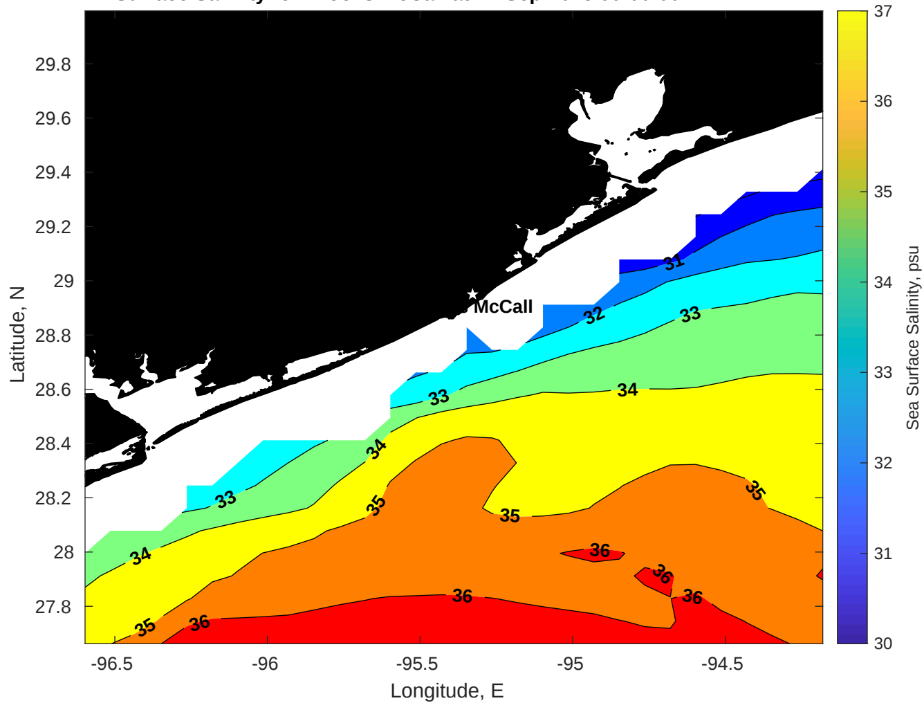
Surface Salinity for Brooks McCall at 17-Sep-2025 00:00:00
