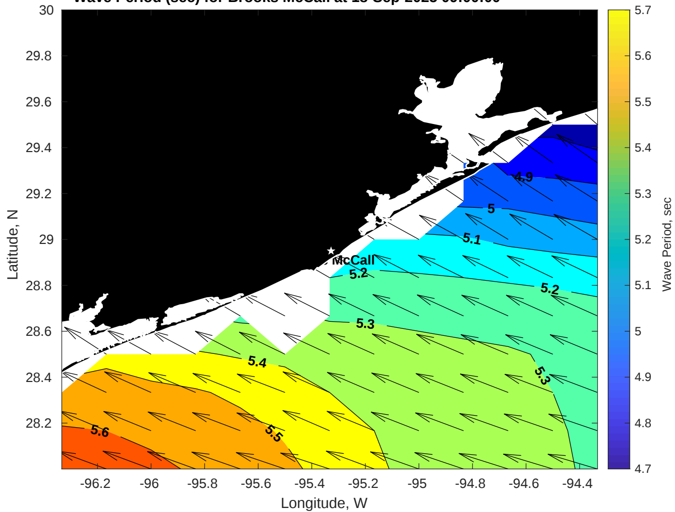
Wave Period (sec) for Brooks McCall at 18-Sep-2025 09:00:00
