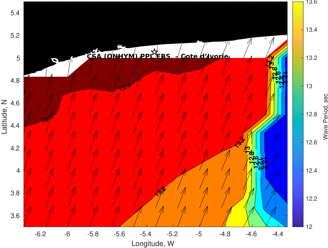
Wave Period (sec) for CSA (ONHYM) PPL EBS - Cote d'Ivoire at 18-Sep-2025 09:00:00
