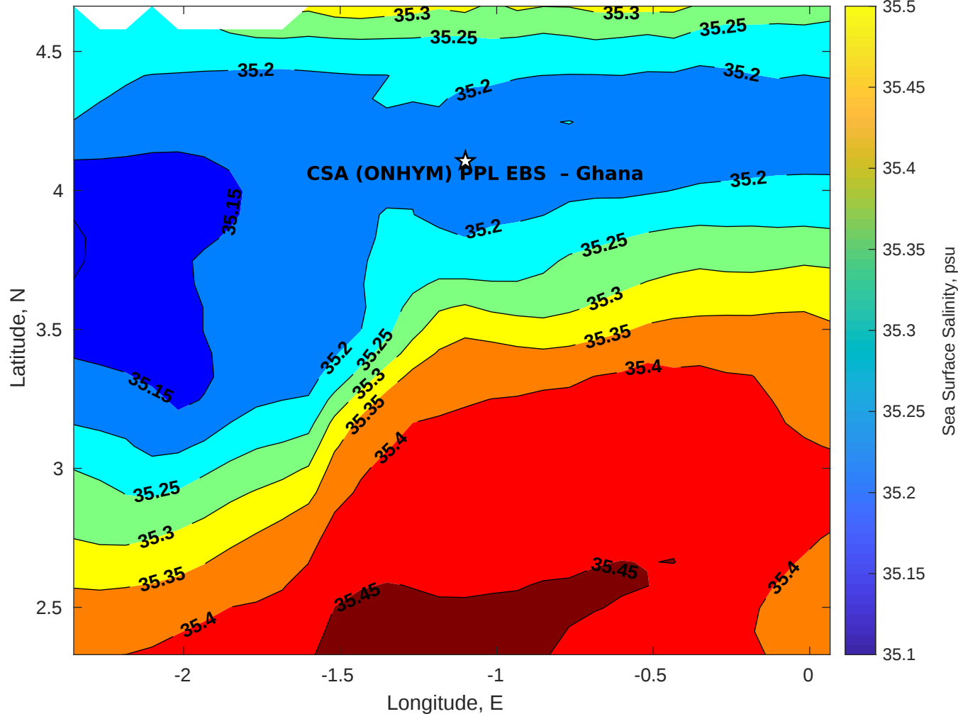
Surface Salinity for CSA (ONHYM) PPL EBS - Ghana at 17-Sep-2025 00:00:00
