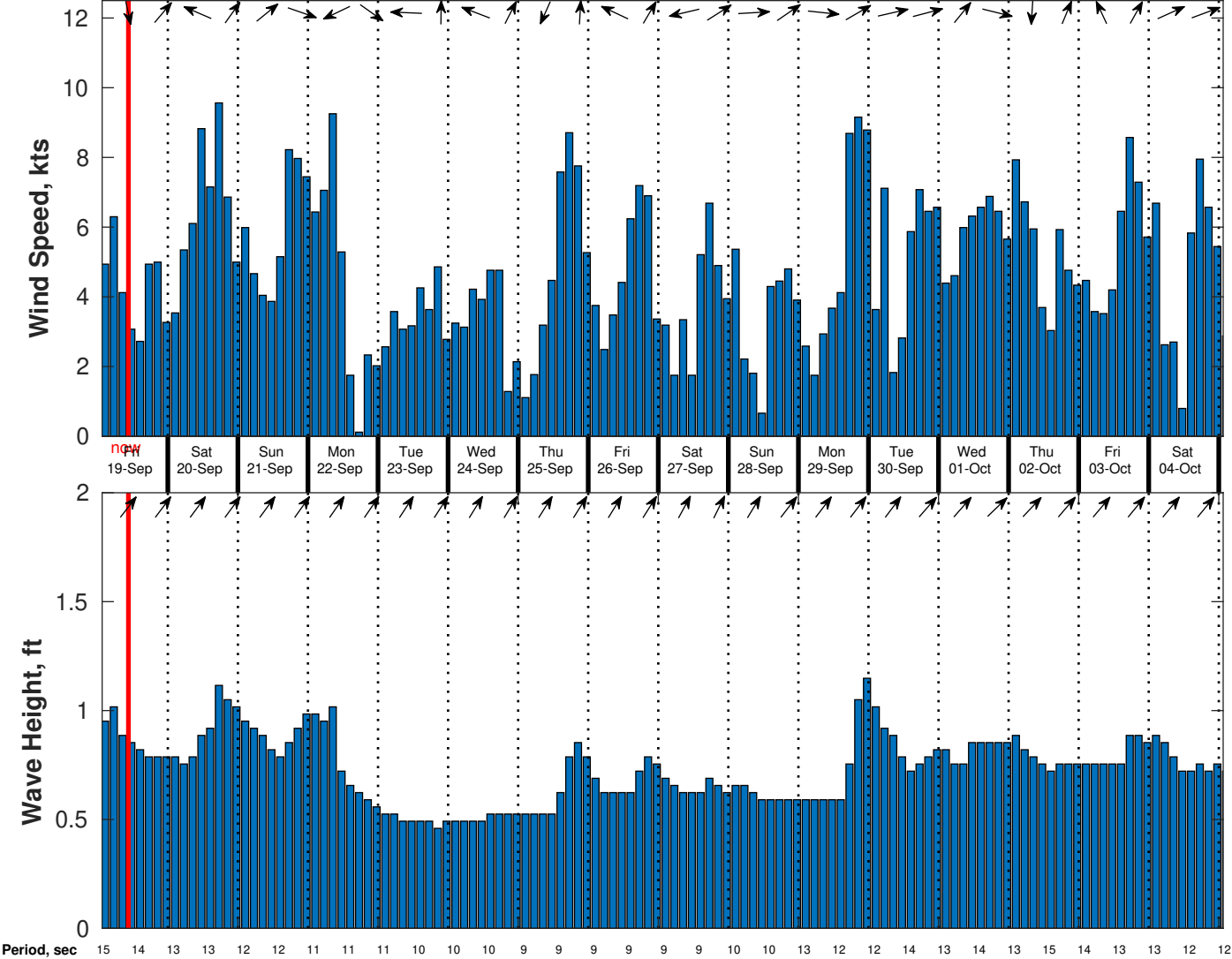
Wind & Wave Forecast for CSA (ONHYM) PPL EBS - Guinea from 18-Sep-2025 01:00:00 to 04-Oct-2025 01:00:00
