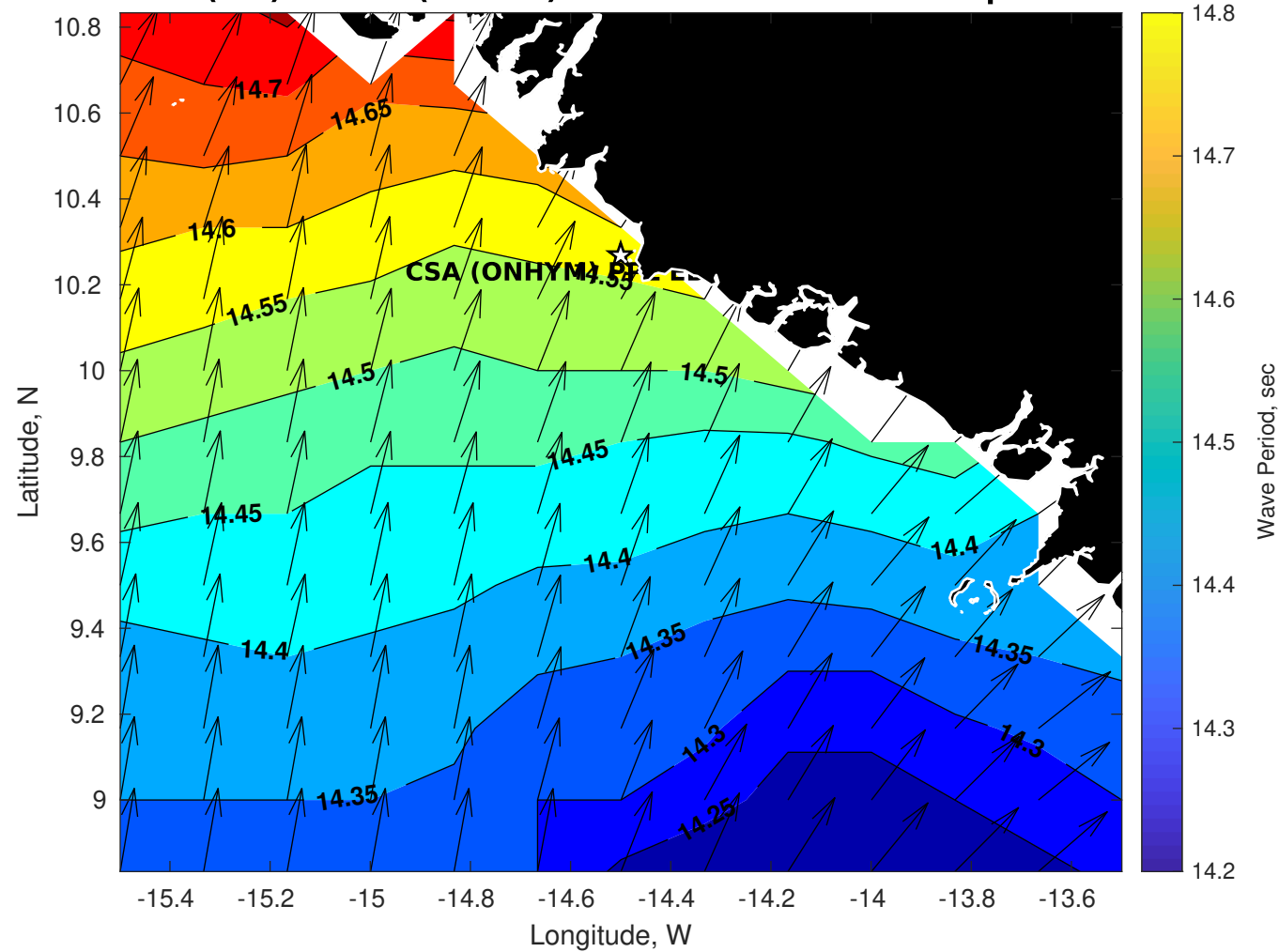
Wave Period (sec) for CSA (ONHYM) PPL EBS - Guinea at 18-Sep-2025 09:00:00
