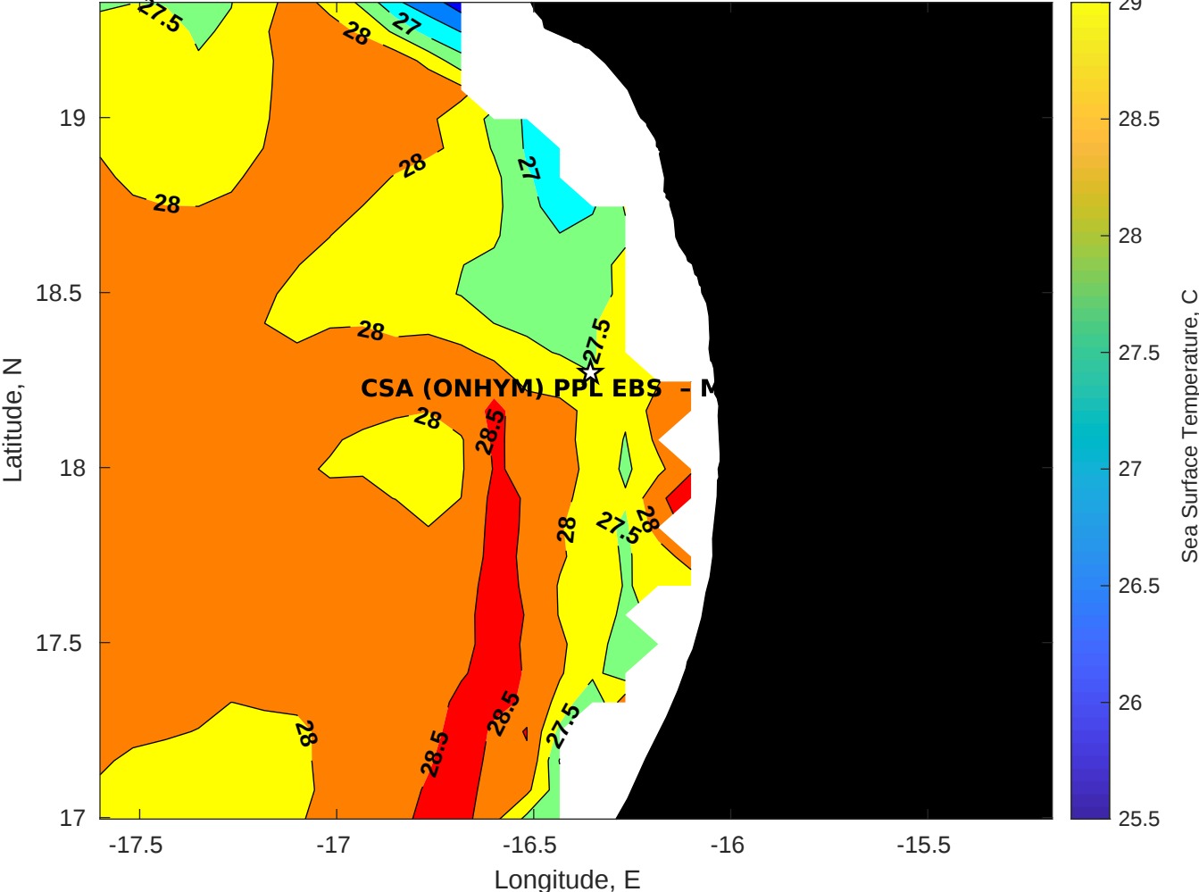
SST for CSA (ONHYM) PPL EBS - Mauritania at 17-Sep-2025 00:00:00
