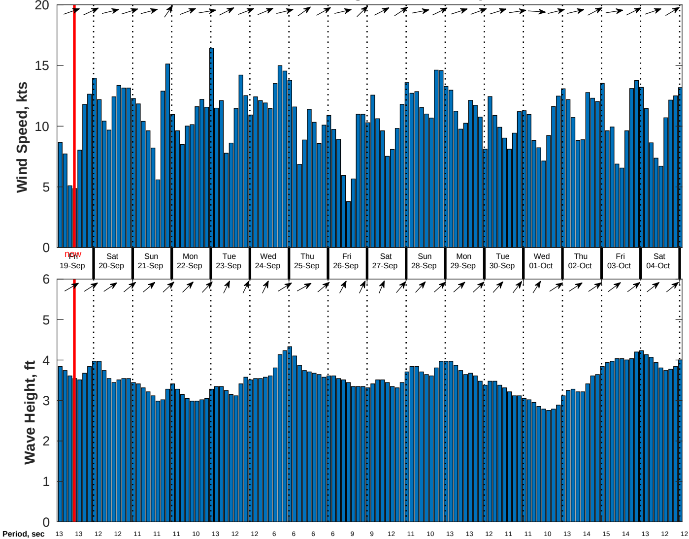
Wind & Wave Forecast for CSA (ONHYM) PPL EBS - Nigeria from 18-Sep-2025 02:00:00 to 04-Oct-2025 02:00:00
