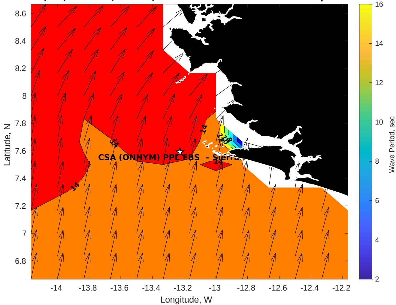
Wave Period (sec) for CSA (ONHYM) PPL EBS - Sierra Leone at 18-Sep-2025 09:00:00
