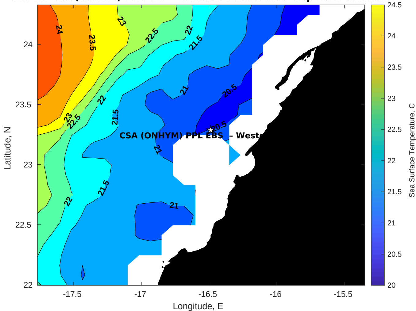
SST for CSA (ONHYM) PPL EBS - Western Sahara at 17-Sep-2025 00:00:00
