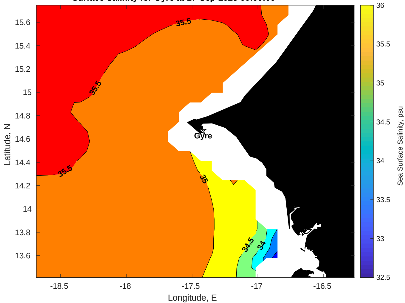
Surface Salinity for Gyre at 17-Sep-2025 00:00:00
