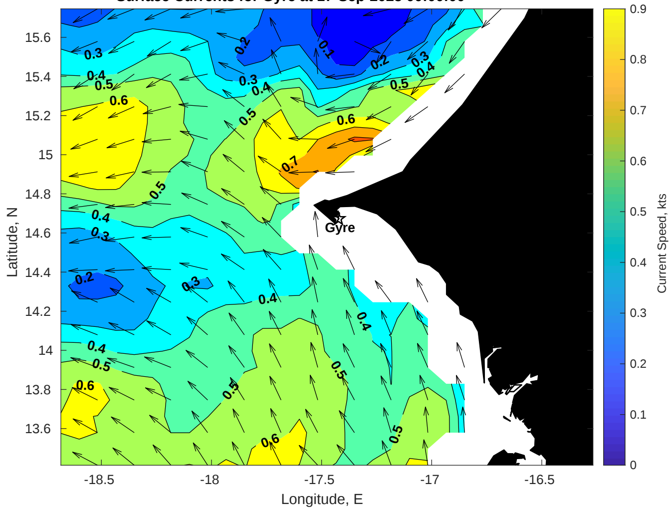
Surface Currents for Gyre at 17-Sep-2025 00:00:00
