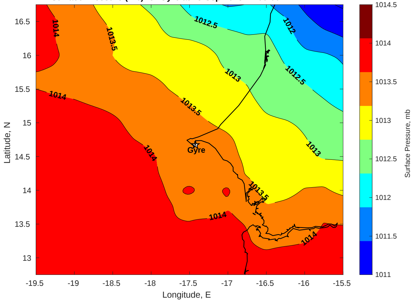
Surface Pressure (mb) for Gyre at 18-Sep-2025 12:00:00
