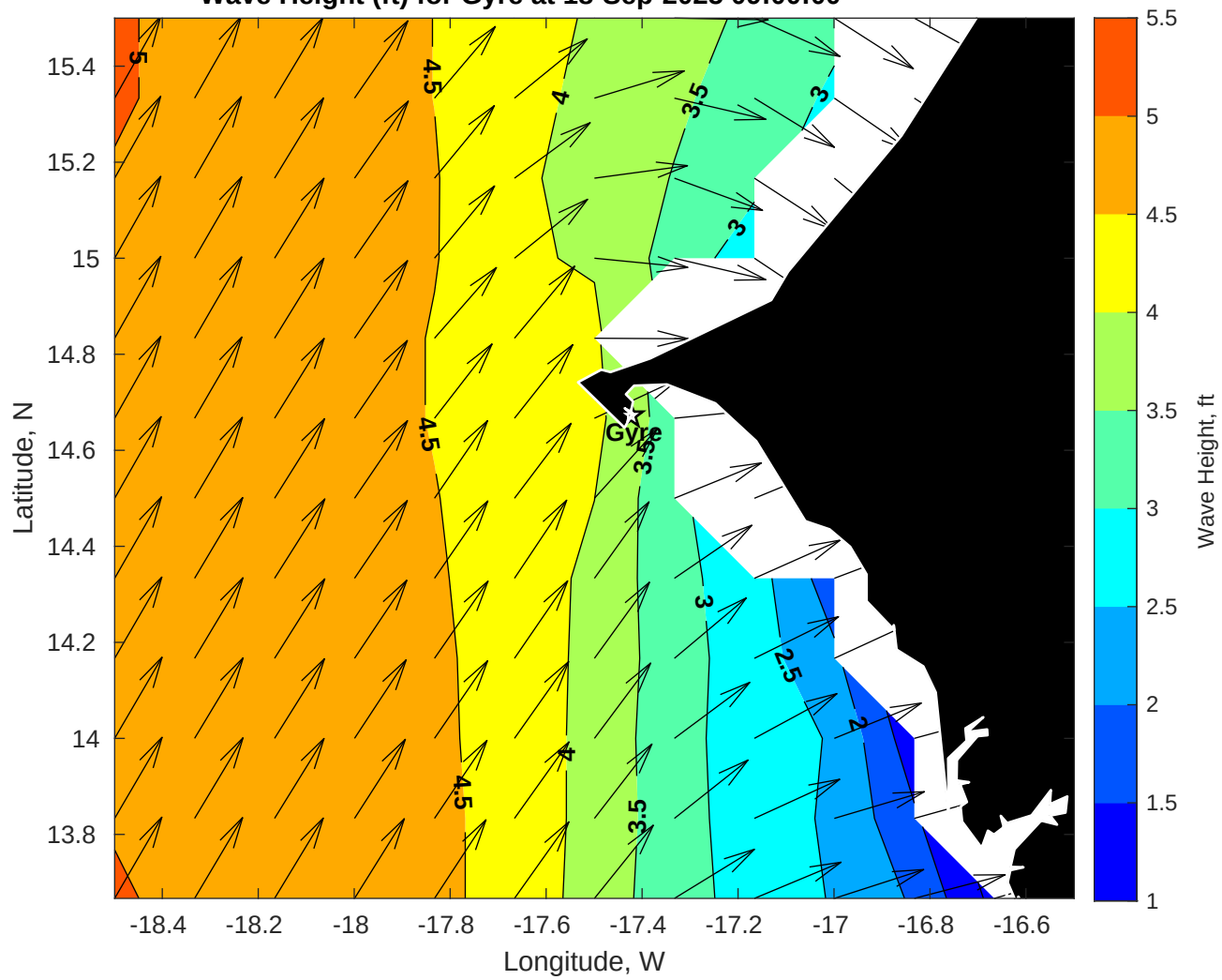
Wave Height (ft) for Gyre at 18-Sep-2025 09:00:00
