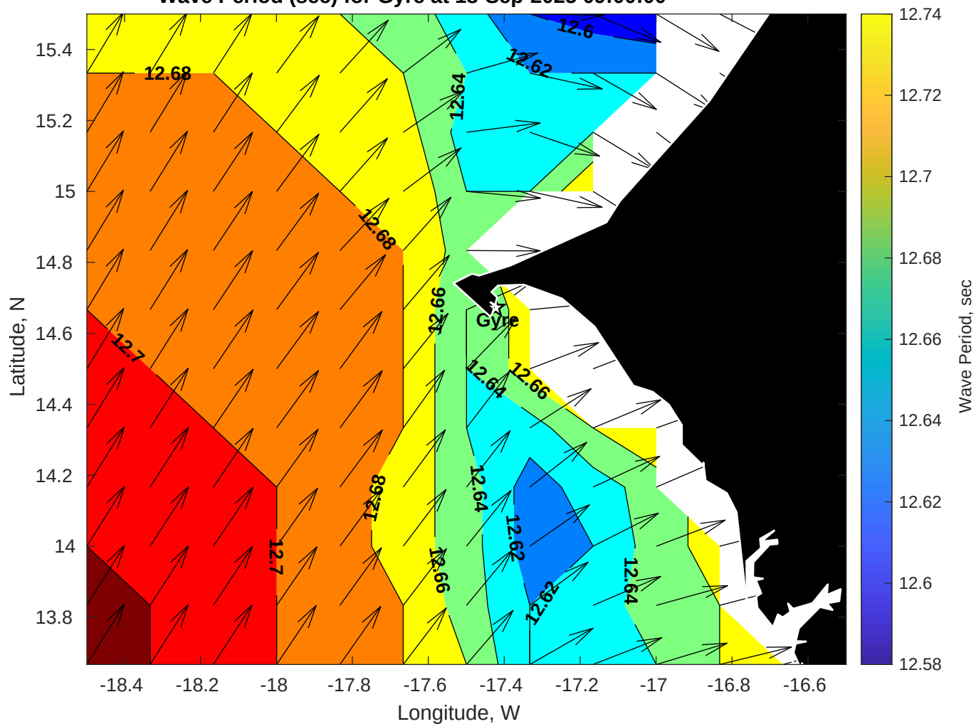
Wave Period (sec) for Gyre at 18-Sep-2025 09:00:00
