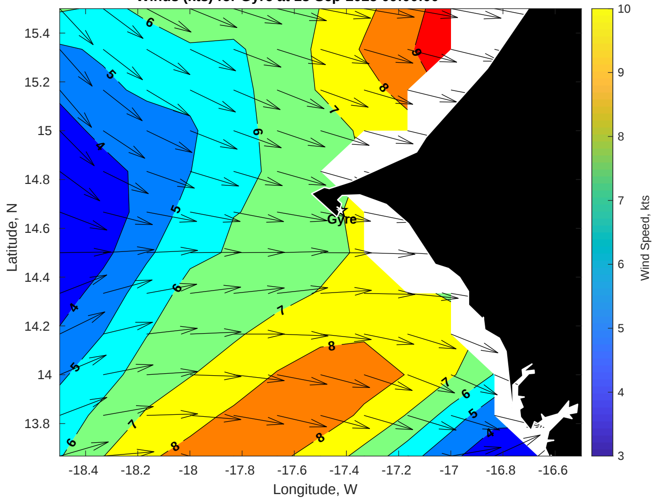
Winds (kts) for Gyre at 18-Sep-2025 09:00:00
