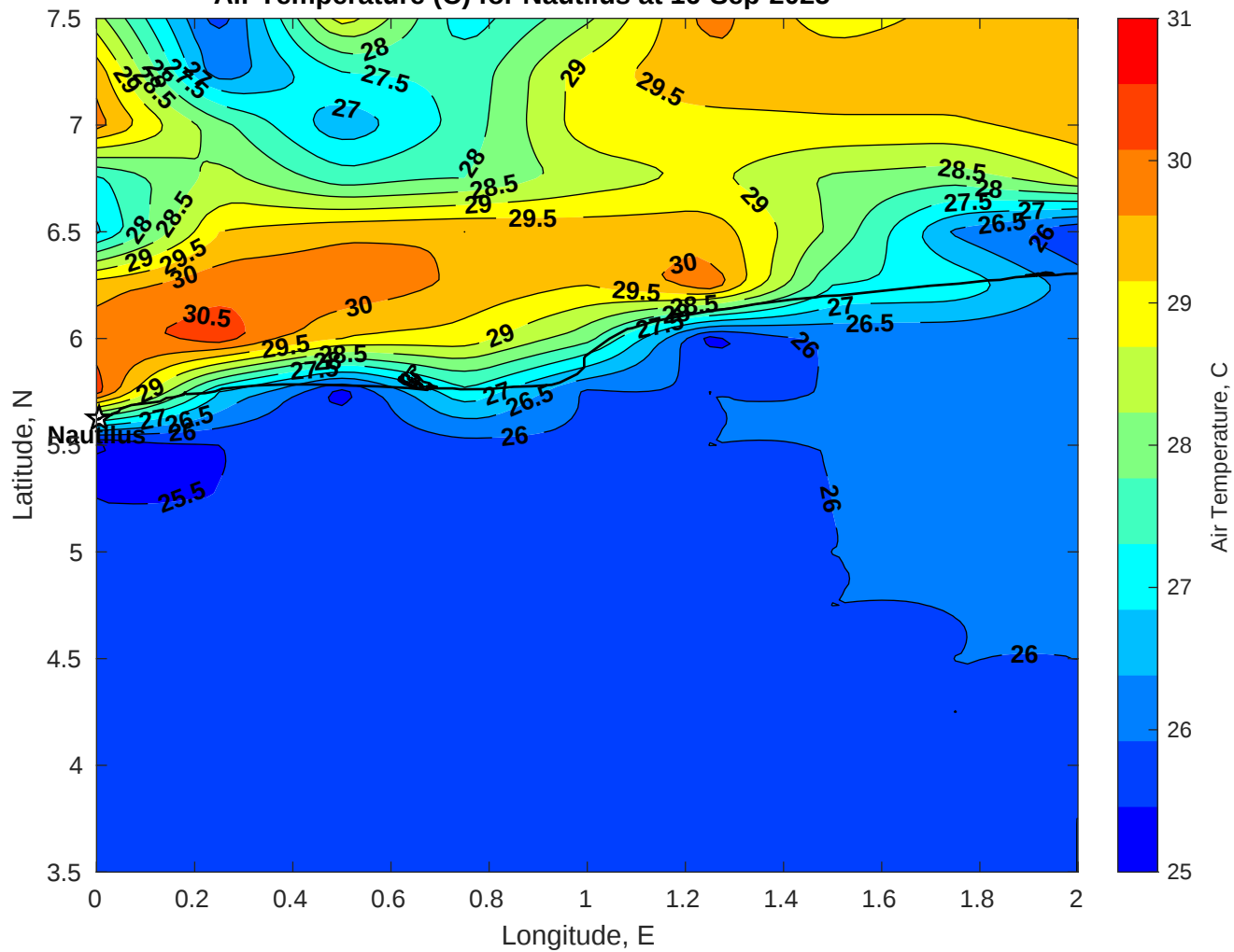
Air Temperature (C) for Nautilus at 16-Sep-2025
