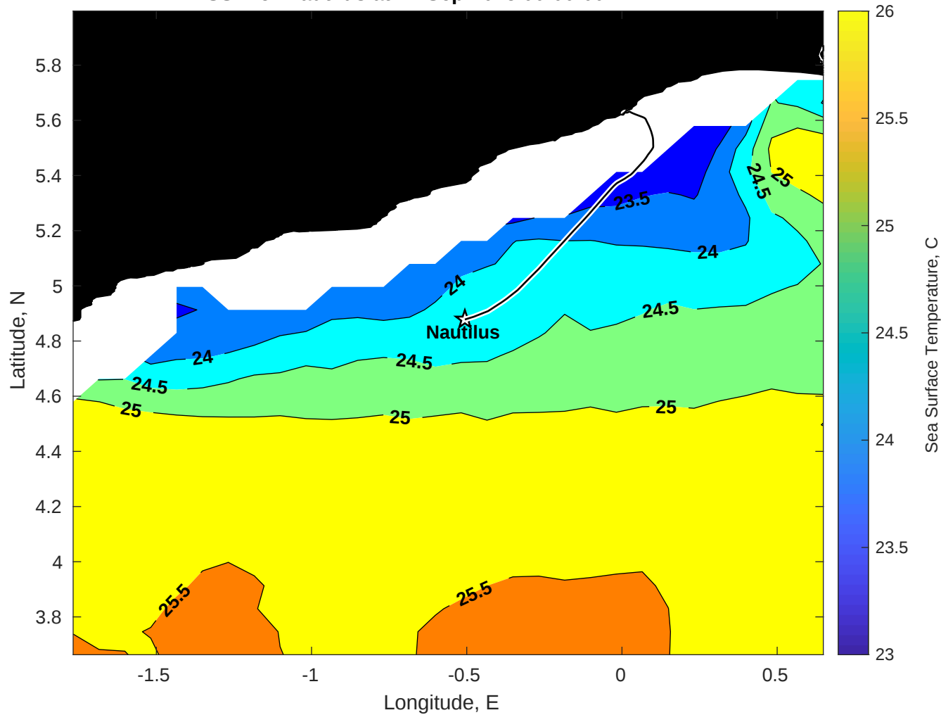
SST for Nautilus at 17-Sep-2025 00:00:00
