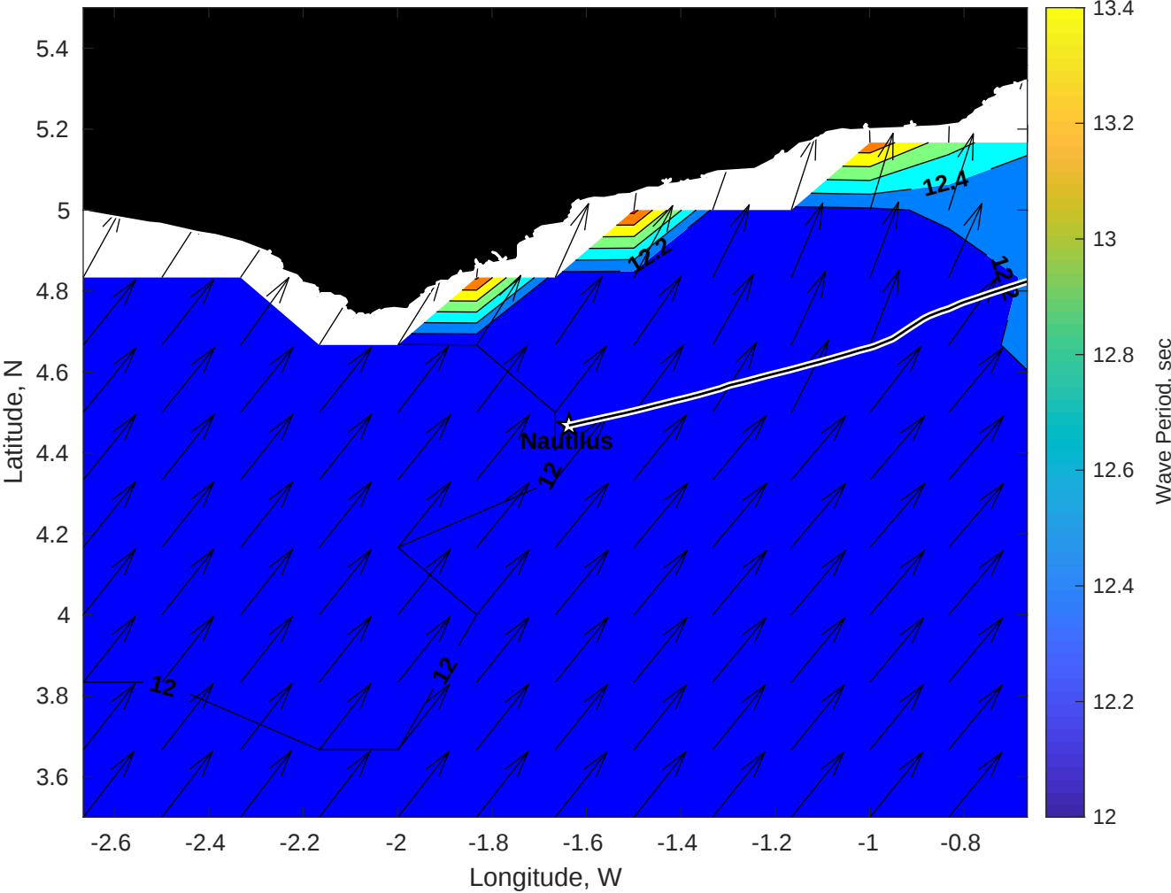
Wave Period (sec) for Nautilus at 18-Sep-2025 09:00:00
