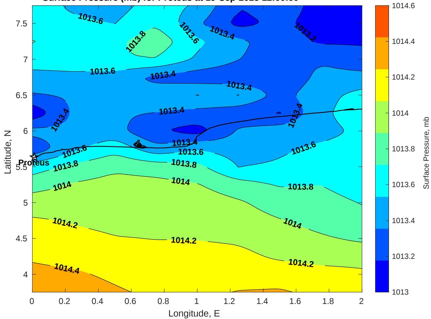
Surface Pressure (mb) for Proteus at 19-Sep-2025 12:00:00
