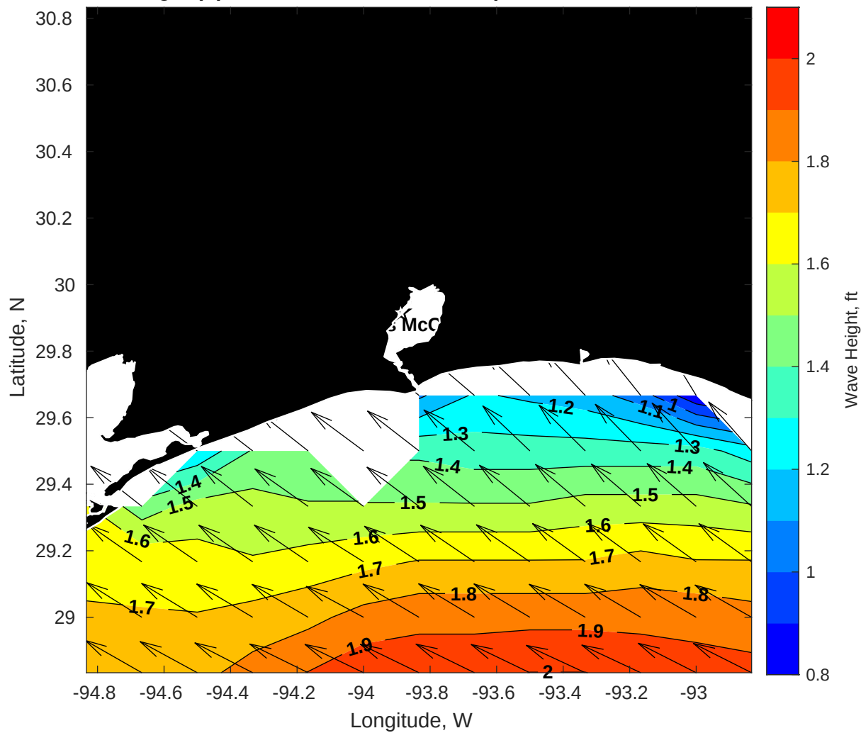
Wave Height (ft) for Brooks McCall at 19-Sep-2025 09:00:00
