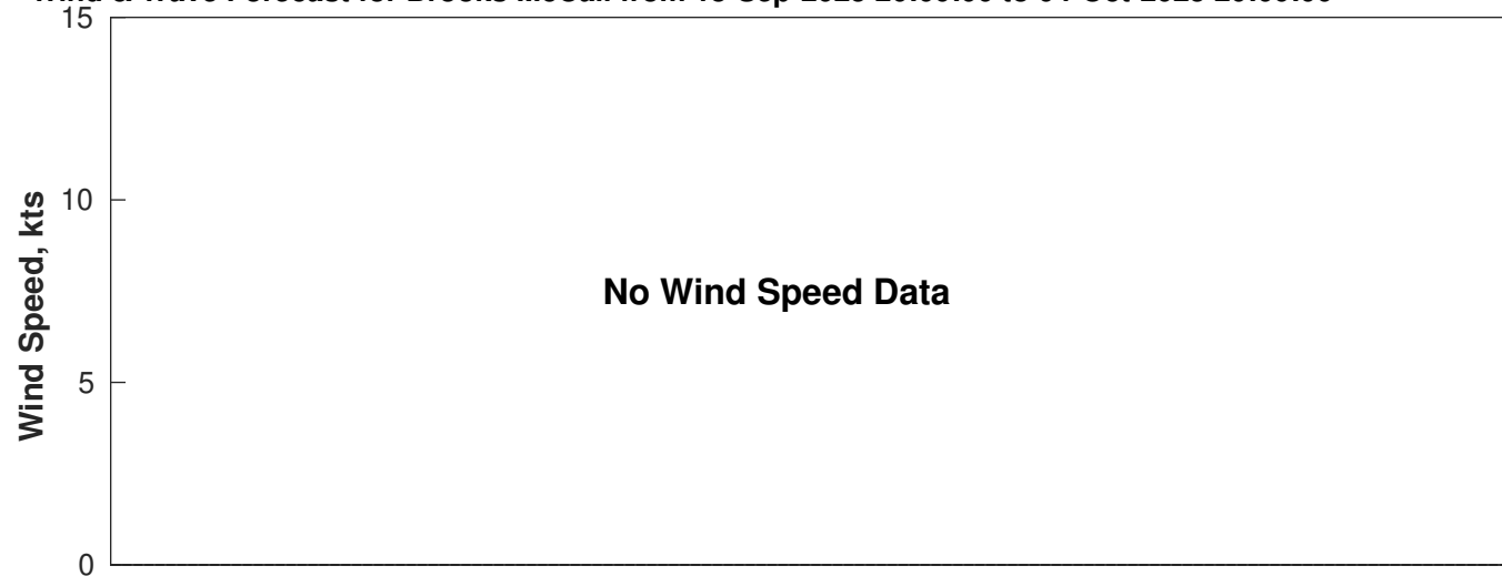
Wind & Wave Forecast for Brooks McCall from 18-Sep-2025 20:00:00 to 04-Oct-2025 20:00:00
