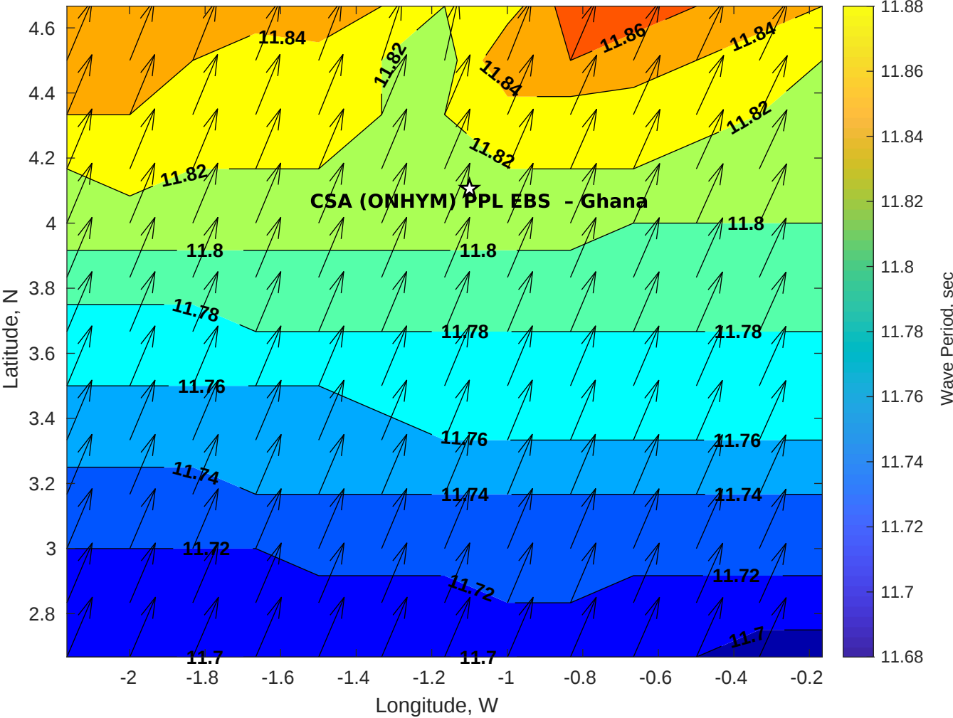
Wave Period (sec) for CSA (ONHYM) PPL EBS - Ghana at 19-Sep-2025 09:00:00
