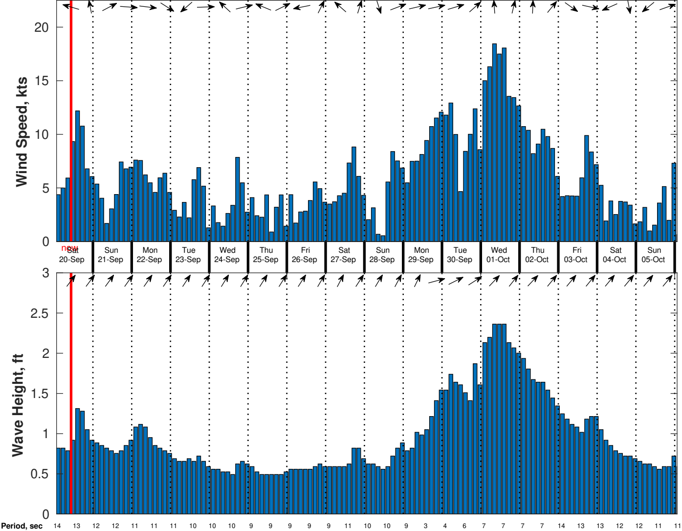
Wind & Wave Forecast for CSA (ONHYM) PPL EBS - Guinea from 19-Sep-2025 01:00:00 to 05-Oct-2025 01:00:00
