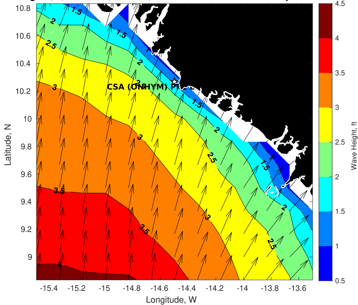
Wave Height (ft) for CSA (ONHYM) PPL EBS - Guinea at 19-Sep-2025 09:00:00
