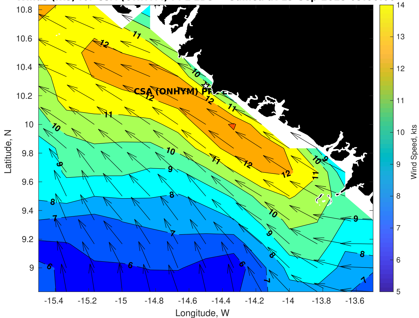
Winds (kts) for CSA (ONHYM) PPL EBS - Guinea at 19-Sep-2025 09:00:00
