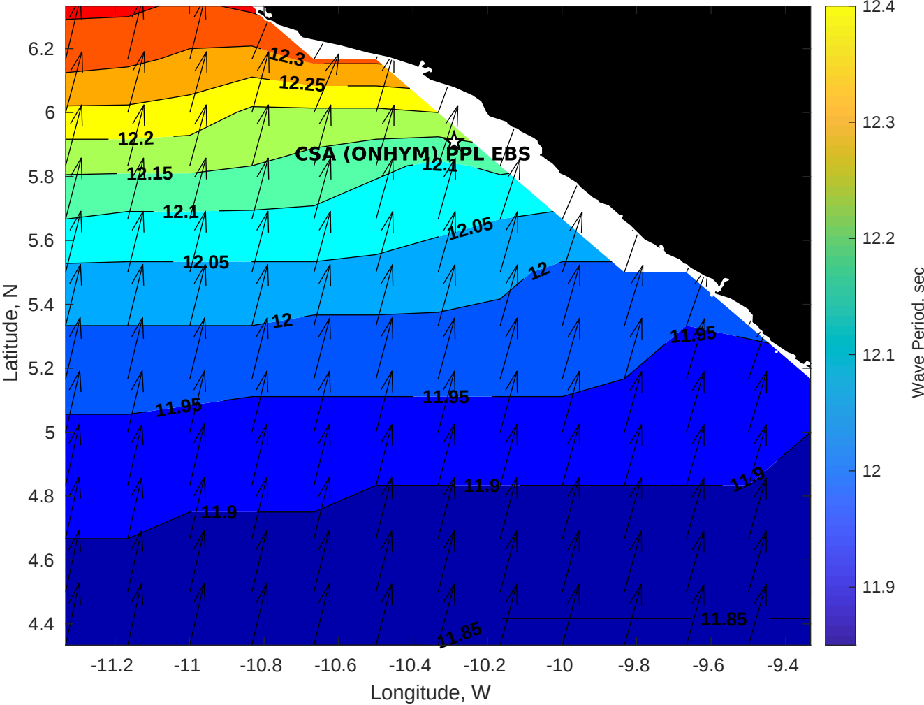
Wave Period (sec) for CSA (ONHYM) PPL EBS - Liberia at 19-Sep-2025 09:00:00
