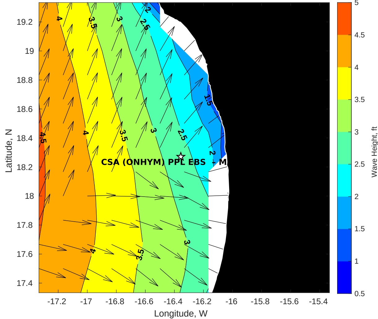
Wave Height (ft) for CSA (ONHYM) PPL EBS - Mauritania at 19-Sep-2025 09:00:00
