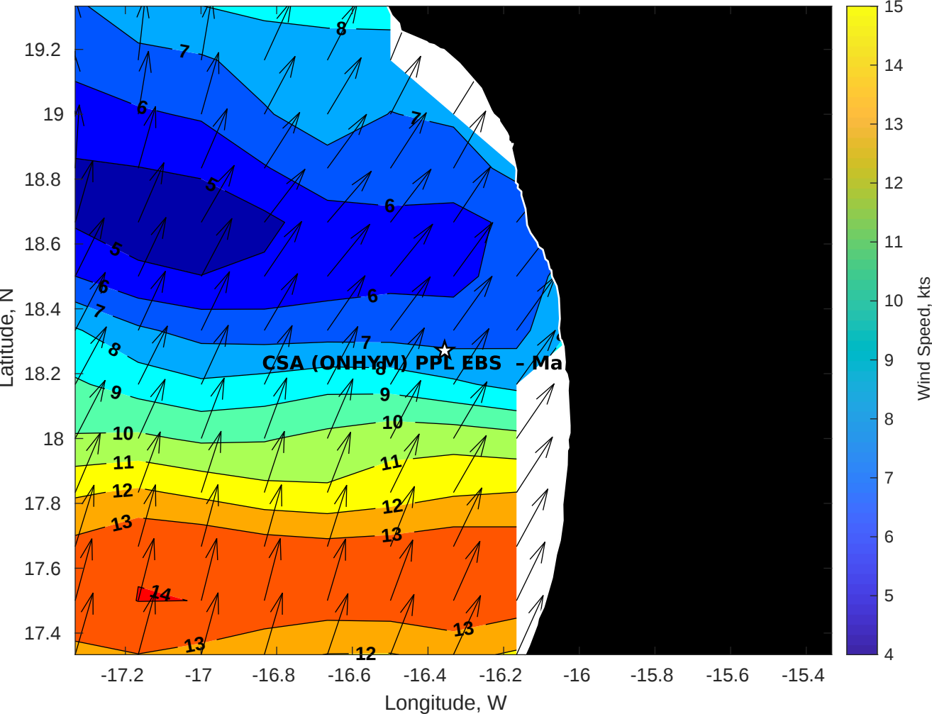
Winds (kts) for CSA (ONHYM) PPL EBS - Mauritania at 19-Sep-2025 09:00:00
