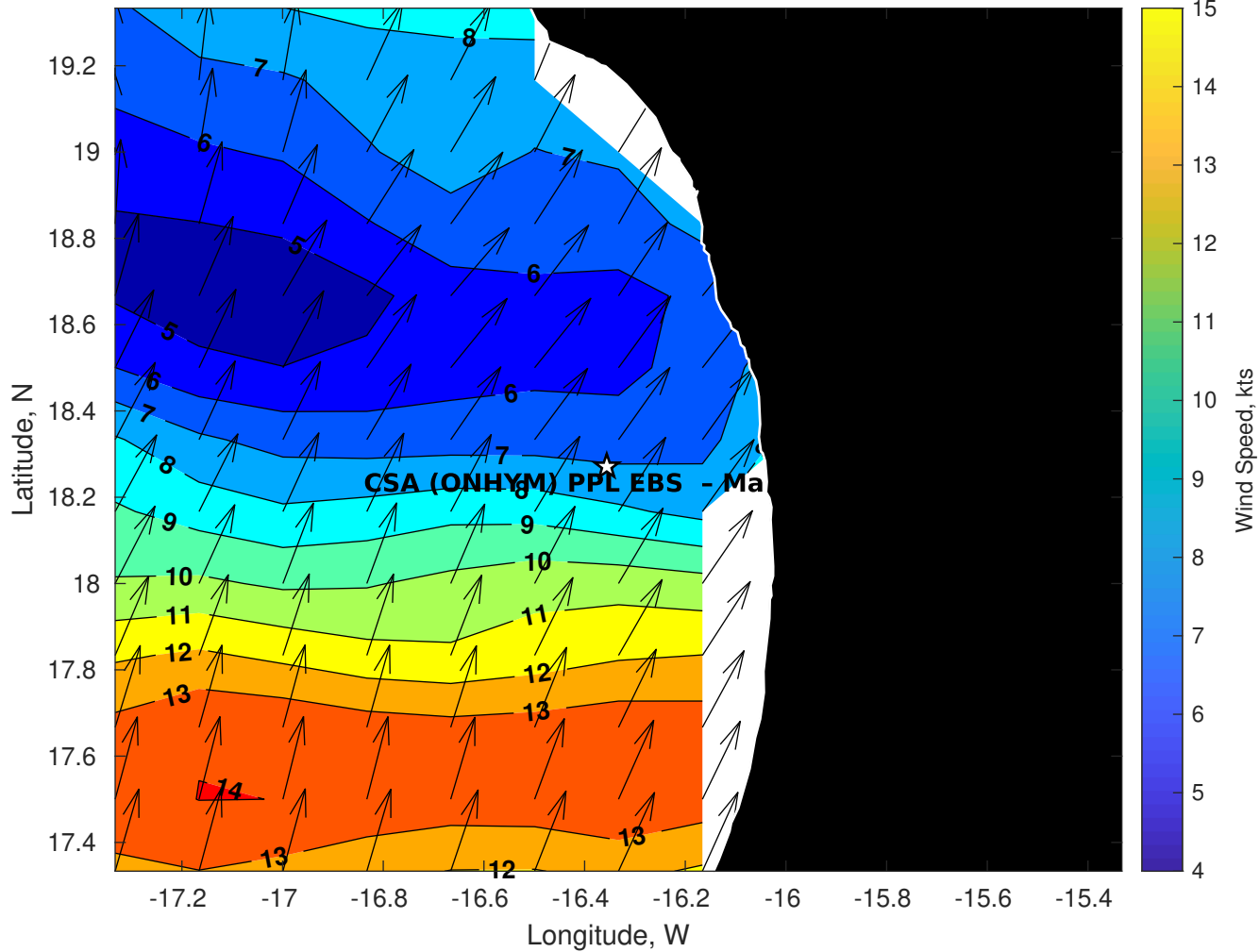
Winds (kts) for CSA (ONHYM) PPL EBS - Mauritania at 19-Sep-2025 09:00:00
