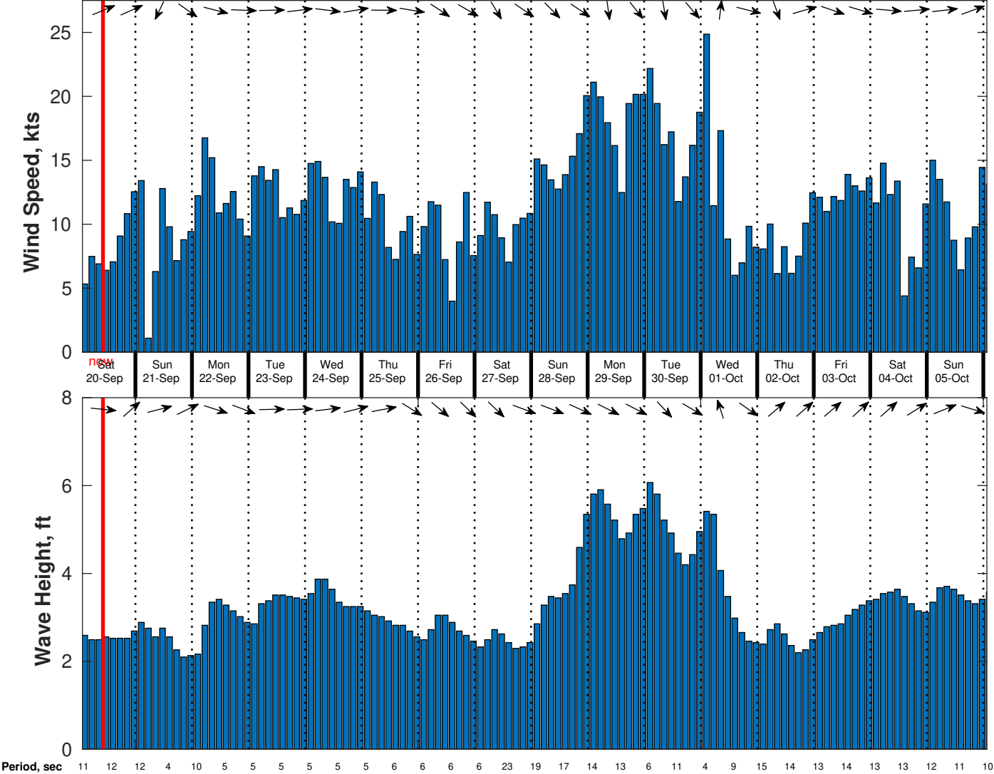
Wind & Wave Forecast for CSA (ONHYM) PPL EBS - Mauritania from 19-Sep-2025 01:00:00 to 05-Oct-2025 01:00:00
