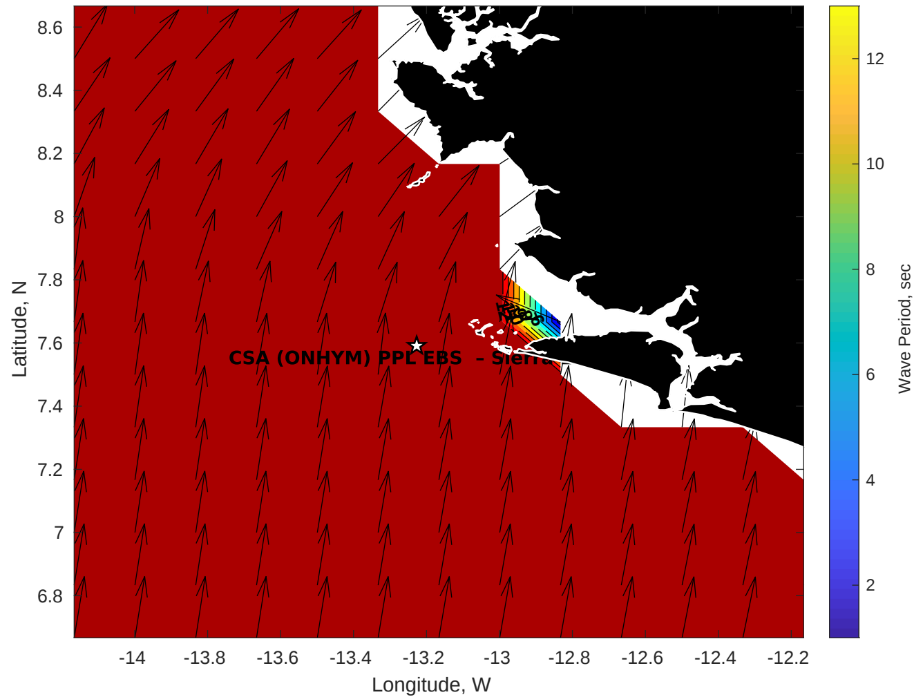
Wave Period (sec) for CSA (ONHYM) PPL EBS - Sierra Leone at 19-Sep-2025 09:00:00
