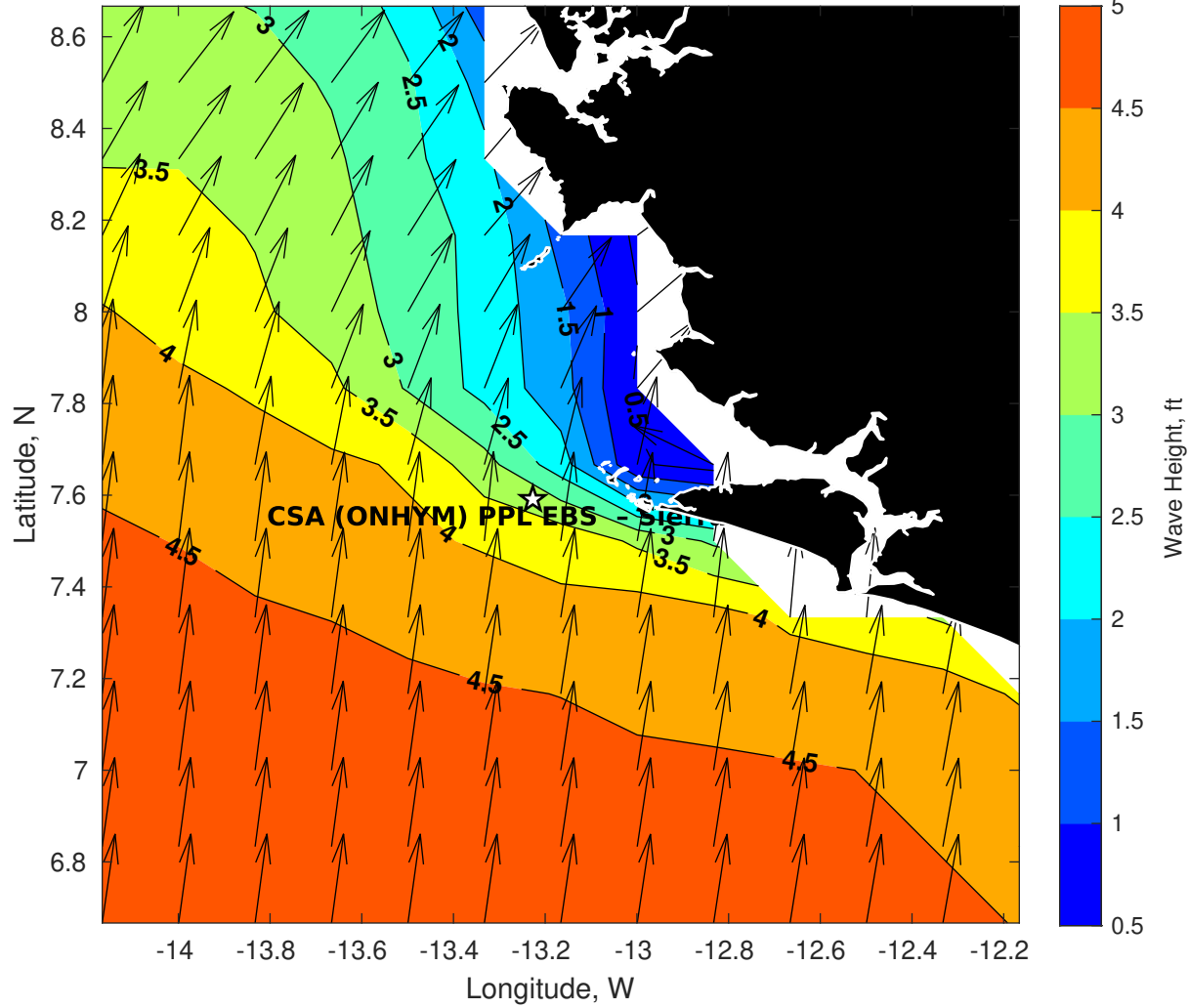
Wave Height (ft) for CSA (ONHYM) PPL EBS - Sierra Leone at 19-Sep-2025 09:00:00
