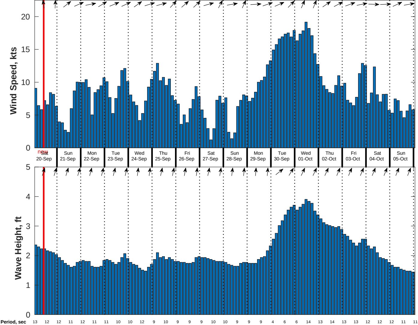
Wind & Wave Forecast for CSA (ONHYM) PPL EBS - Sierra Leone from 19-Sep-2025 01:00:00 to 05-Oct-2025 01:00:00
