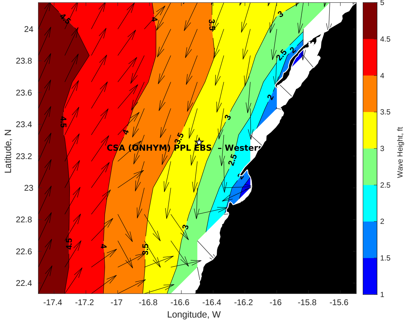
Wave Height (ft) for CSA (ONHYM) PPL EBS - Western Sahara at 19-Sep-2025 09:00:00
