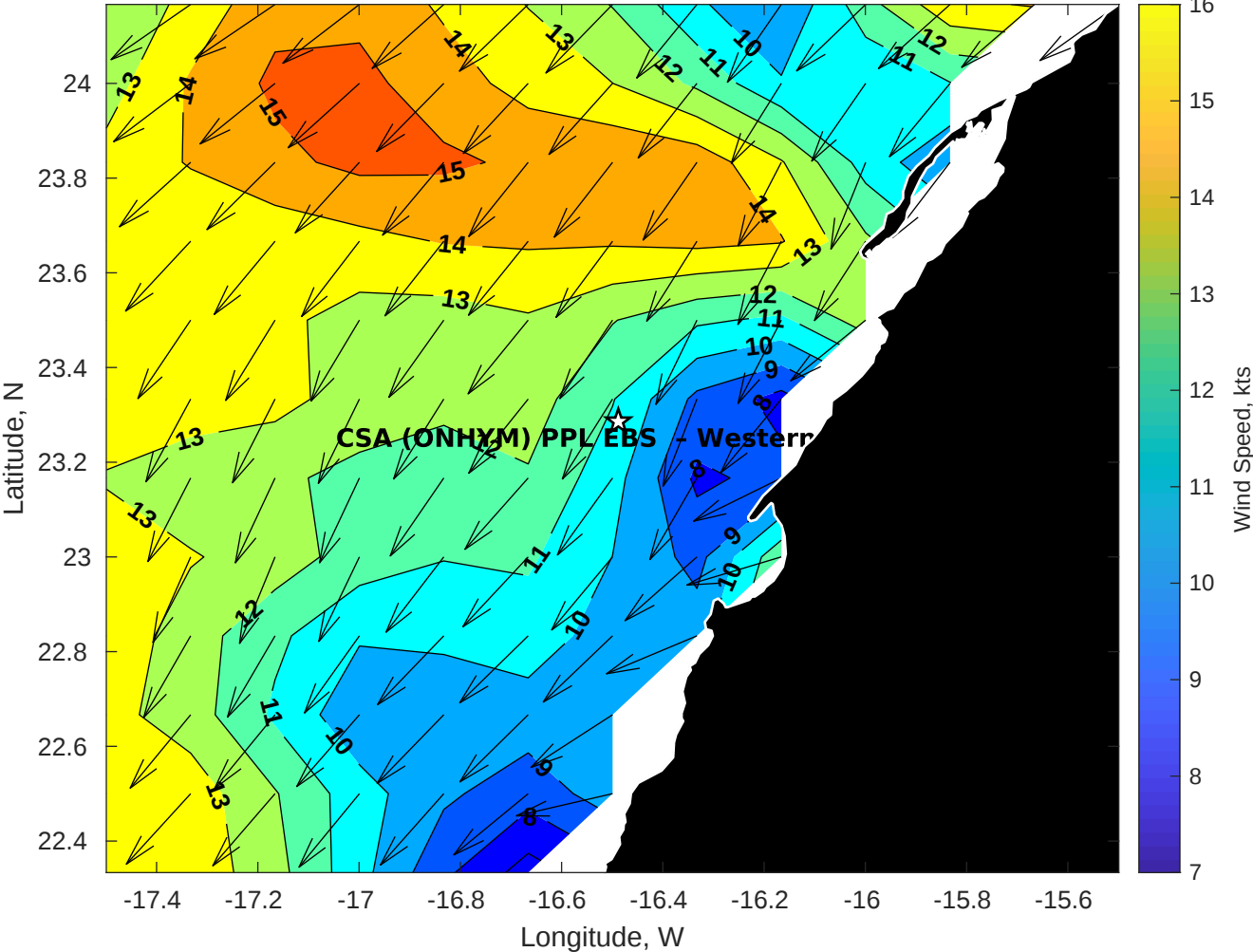
Winds (kts) for CSA (ONHYM) PPL EBS - Western Sahara at 19-Sep-2025 09:00:00
