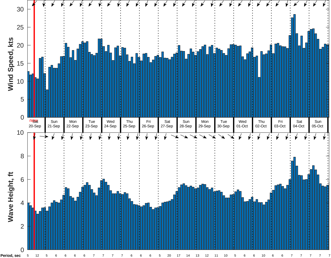
Wind & Wave Forecast for CSA (ONHYM) PPL EBS - Western Sahara from 19-Sep-2025 01:00:00 to 05-Oct-2025 01:00:00
