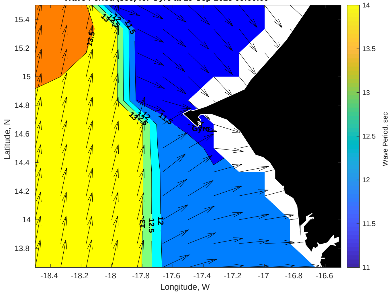
Wave Period (sec) for Gyre at 19-Sep-2025 09:00:00
